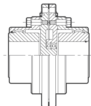
Shear pin gear coupling
