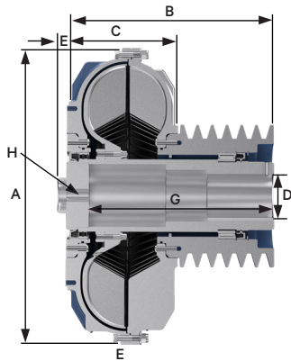
HS.. VP Standard type size 2-12
