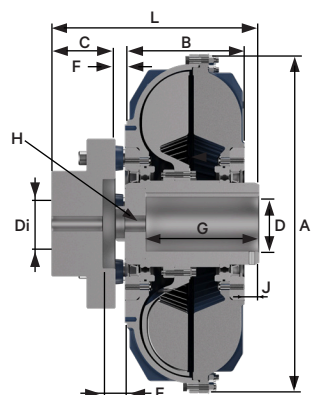
HS.. PF Standard type size 2-13
