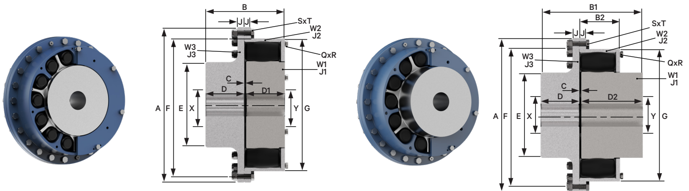
RBI 1.4 - 60 long boss inner member
